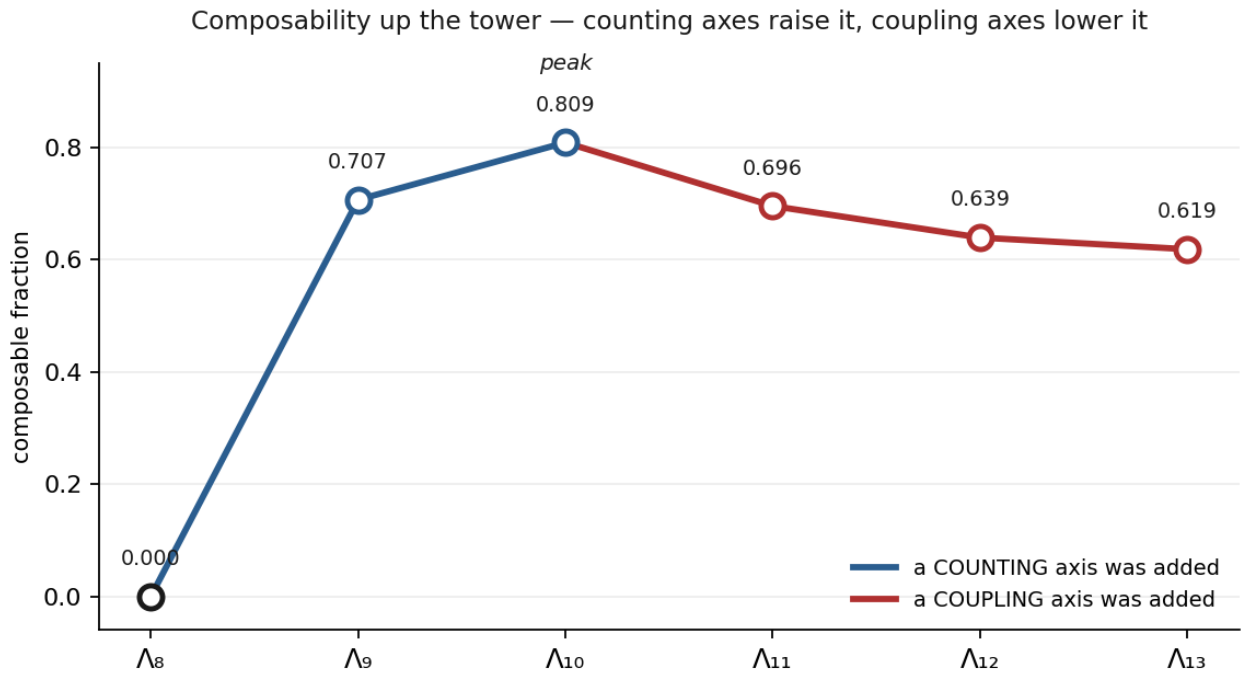
Figure 2. The composable fraction stage by stage. \Lambda_8 composes not at all — four source coordinates against three target. The two counting axes take it to a peak of 0.8087 at \Lambda_{10} ; the three coupling axes lower it every time.
