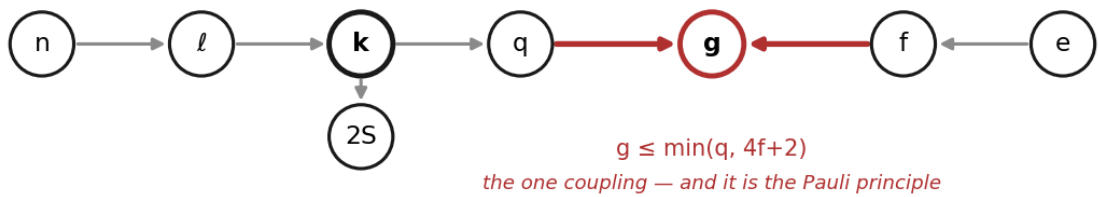
Figure 1. \Lambda_8 's constraint graph. Seven bounds on eight coordinates — a caterpillar with 2S pendant at k. Every edge is a single monotone inequality except one: g takes two parents , and g \leq \min(q, 4f+2) is the only non-product term in the whole expression.
