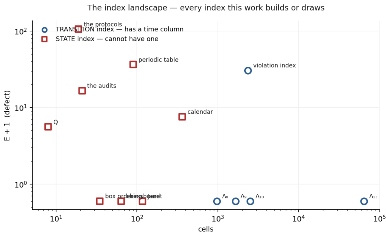
Figure 3. Every index this work builds or draws, by cells against defect. Circles are transition indexes — their cells are moves, so they carry a time column. Squares are state indexes — a cell is one position, and the question of composition does not arise.
