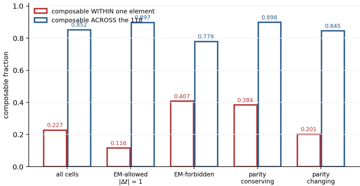
Figure 4. The crossing. Within one atom a dipole-allowed transition is the LEAST likely to be followable; across the 118 elements it is the most. The rule that forbids composition inside an atom is the rule that enables it between atoms.
